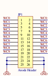
MCA2X16 LED Controller
